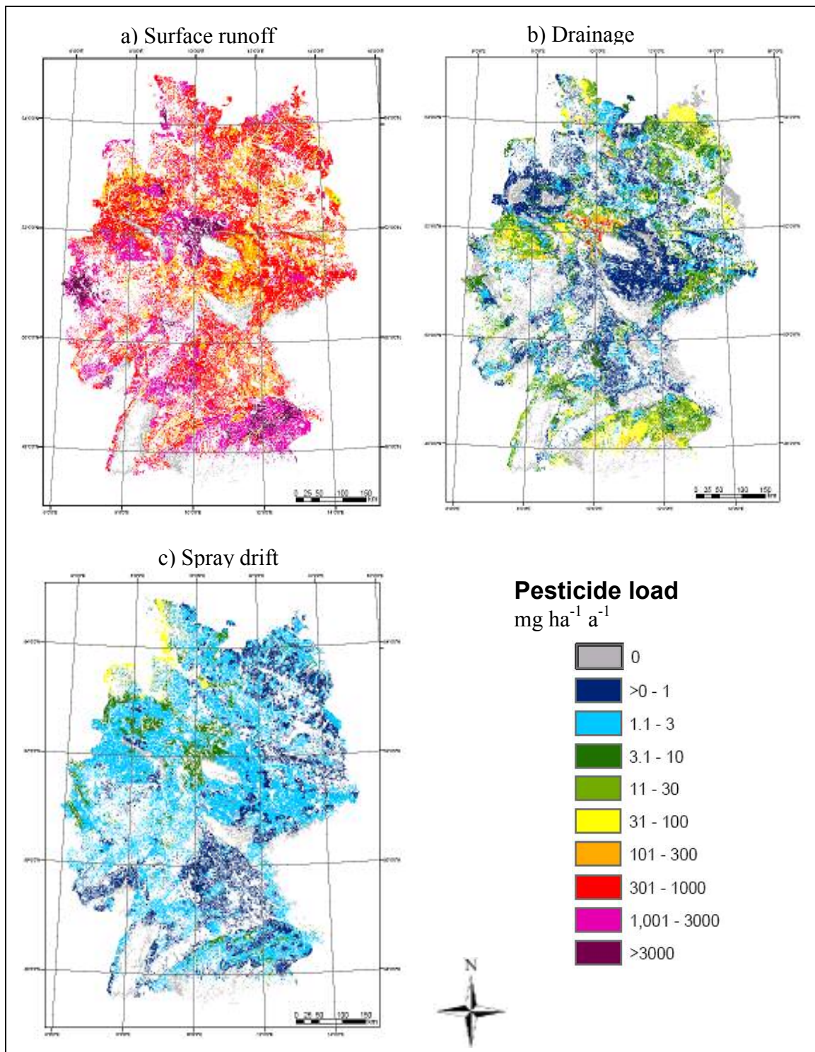
Fig. 1: Spatial distribution of diffuse pesticide losses from field crops (vineyards and orchards excluded) to surface waters in Germany via (a) surface runoff, (b) tile drains, and (c) spray drift according to model DRIPS (reference year 2000; Röpke, 2003; Röpke et al., 2004).
